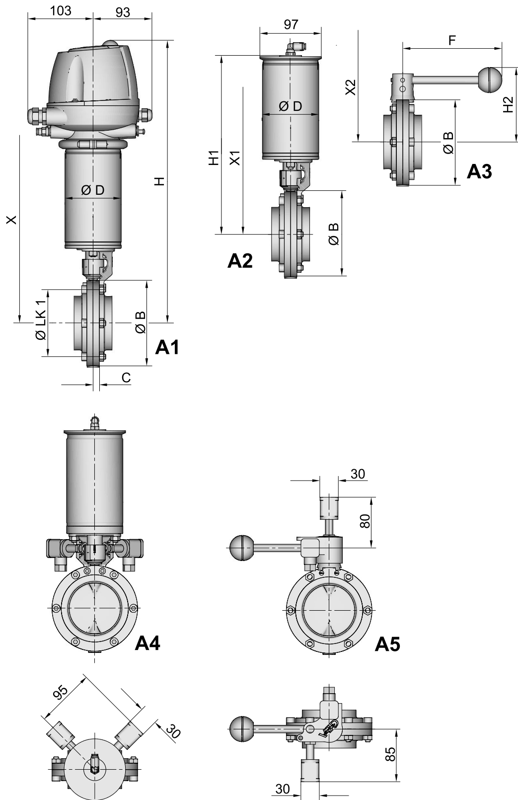
Fig.1: Installation of proximity switches optional / observe removal reserve
